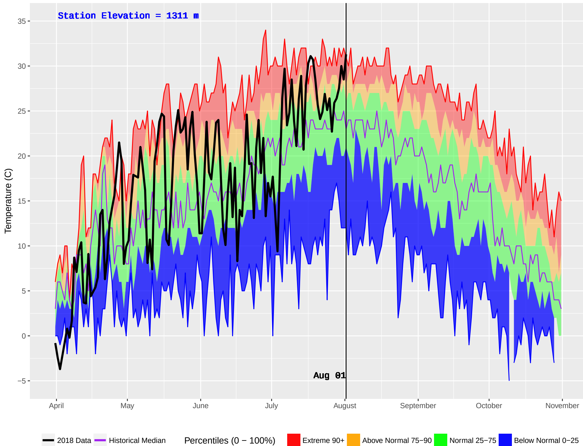
FLATHEAD 2 (418) : Historical (1986–2016) and Current (2018) Daily Temperature
