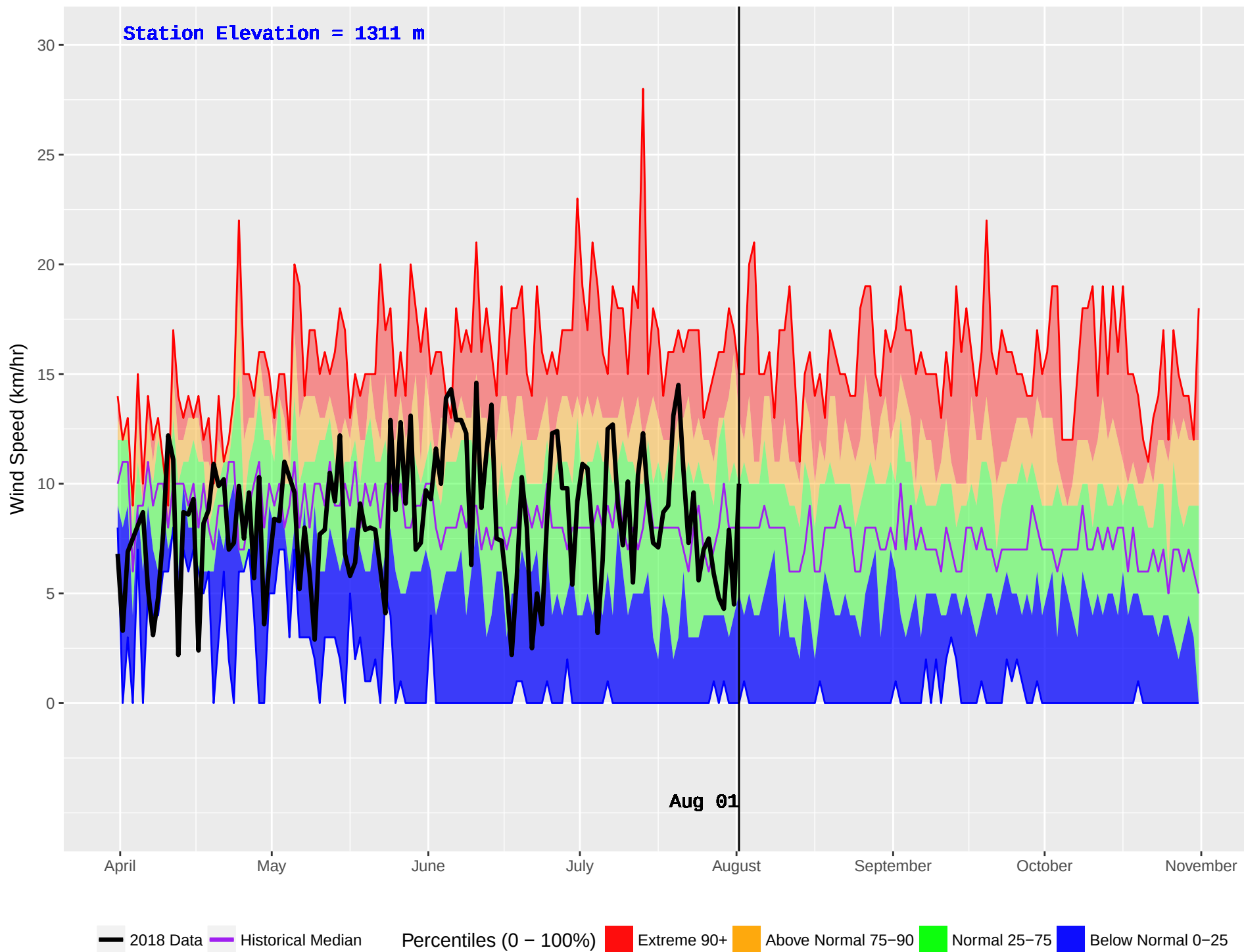
FLATHEAD 2 (418) : Historical (1986–2016) and Current (2018) Daily Wind Speed
