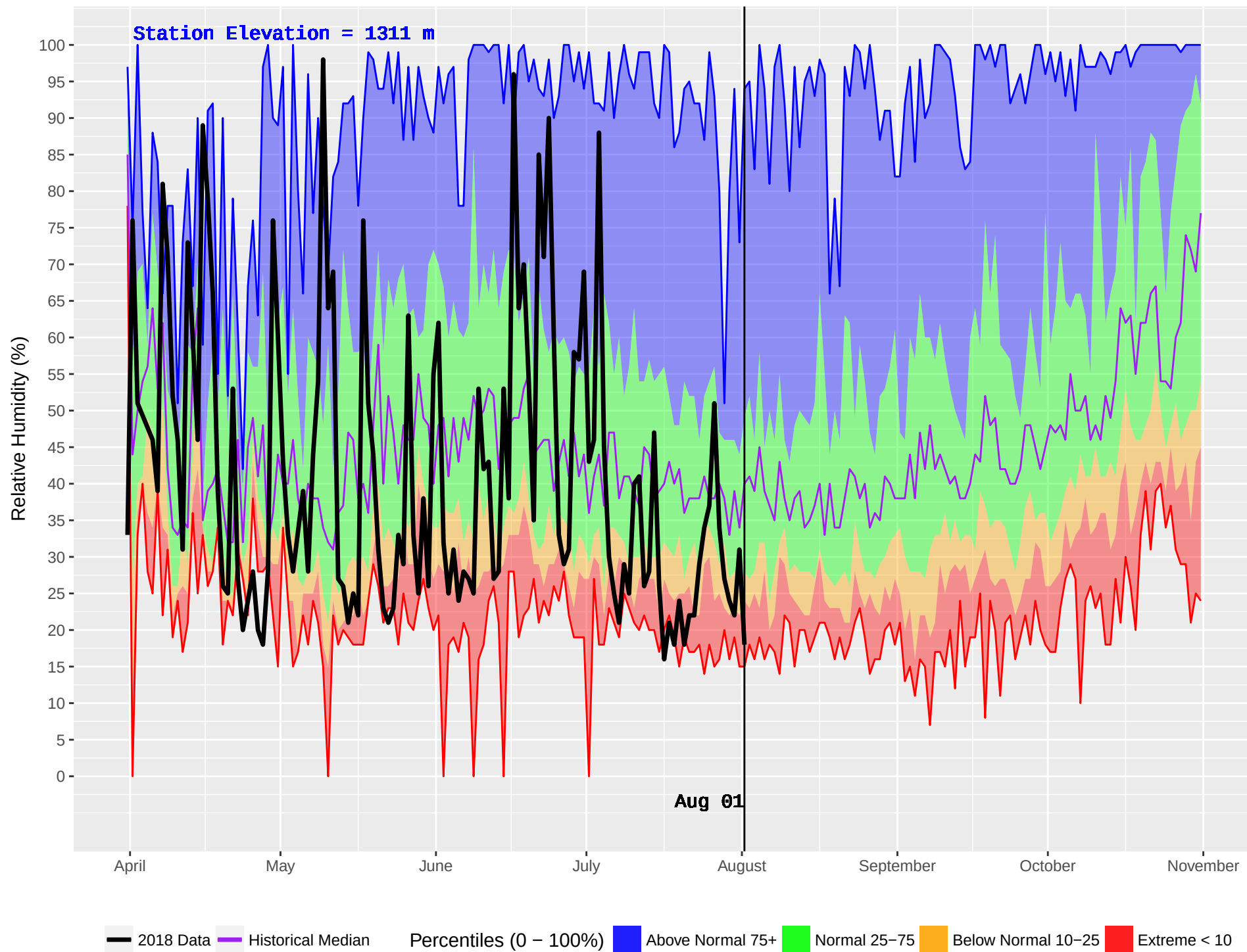
FLATHEAD 2 (418) : Historical (1986–2016) and Current (2018) Daily Relative Humidity
