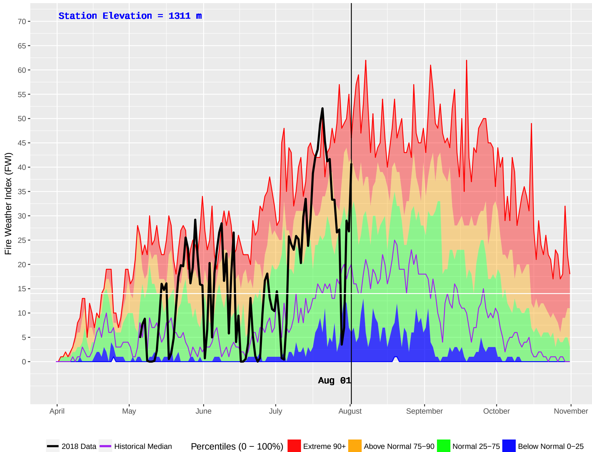
FLATHEAD 2 (418) : Historical (1986–2016) and Current (2018) Daily Fire Weather Index (FWI)
