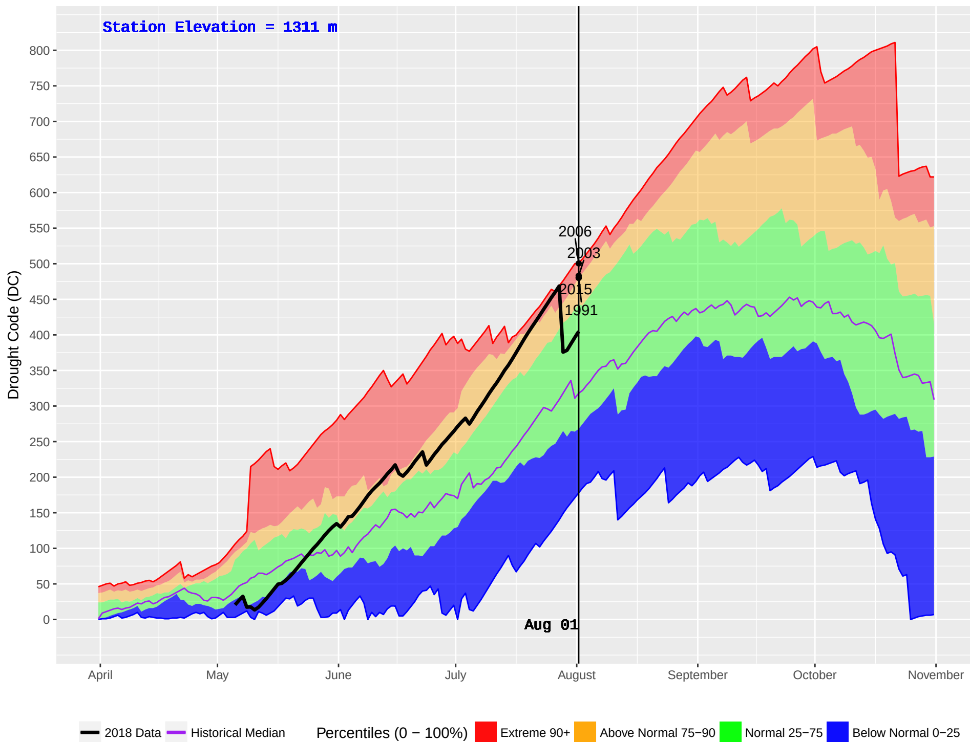
FLATHEAD 2 (418) : Historical (1986–2016) and Current (2018) Daily Drought Code (DC)
