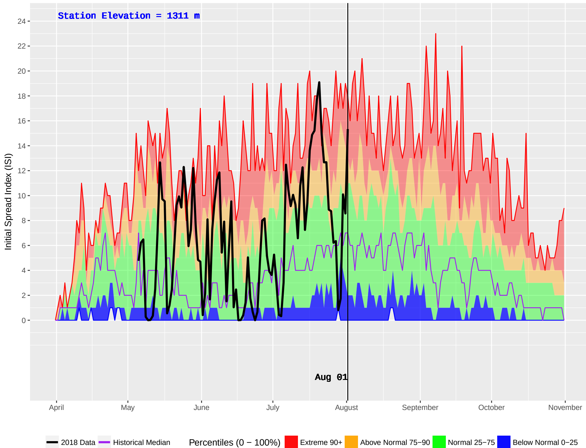
FLATHEAD 2 (418) : Historical (1986–2016) and Current (2018) Daily Initial Spread Index (ISI)
